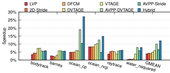
Fig. 25. Speedup of 6 multithreaded workloads.
