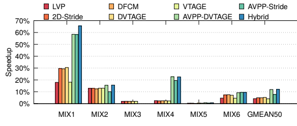
Fig. 26. Speedup of 50 multiprogram mixes of workloads.
