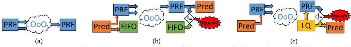
Fig. 7. PRF port pressure in (a) a processor without prediction, (b) a processor with value prediction and (c) our proposal for load value prediction.
