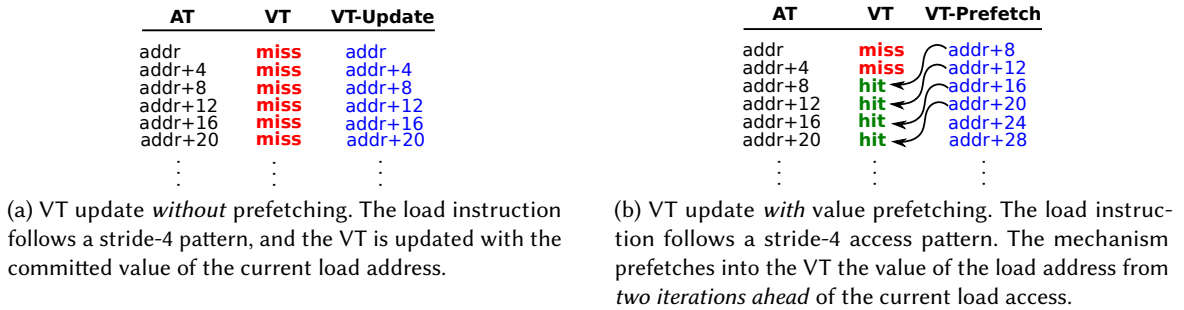
Fig. 3. Examples of (a) VT update without prefetching and (b) VT update with prefetching.
