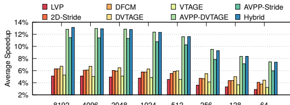
Fig. 17. Impact of predictor size on speedup. For this study, the AT and the VT have the same size in the AVPP predictors, to emphasize the effect of AT size.
