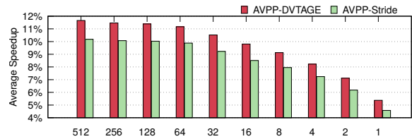
Fig. 18. Impact of VT table size for an AVPP predictor with an AT of 512 entries.
