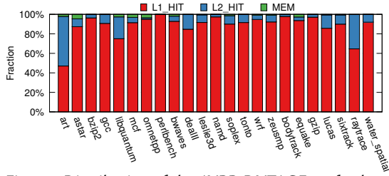
Fig. 13. Distribution of the AVPP-DVTAGE prefetch requests that hit in L1, L2 and main memory.
