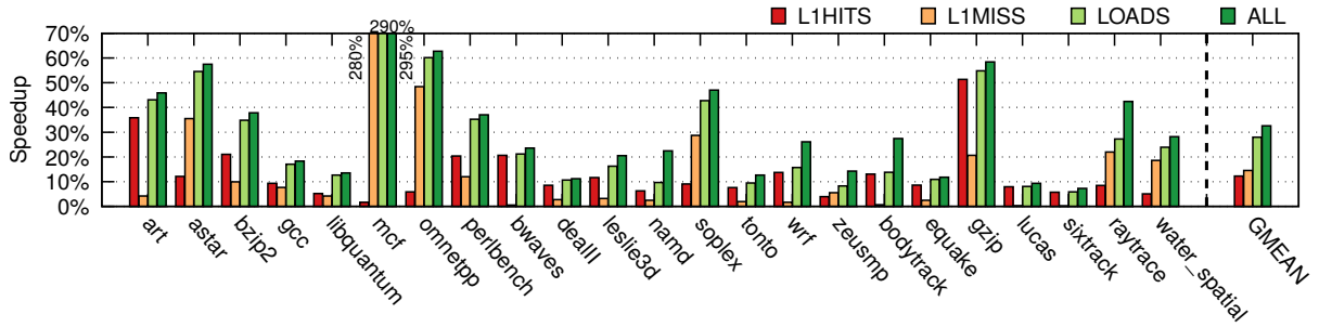
Fig. 1. Speedup when speculating with perfect value prediction on only L1 hit loads (L1HITS); only L1 miss loads (L1MISS); all LOADS; and ALL instructions.
