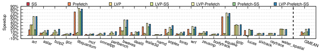
Fig. 23. Interaction between store set prediction (SS), L2 prefetching (Prefetch) and Load Value Prediction (LVP).
