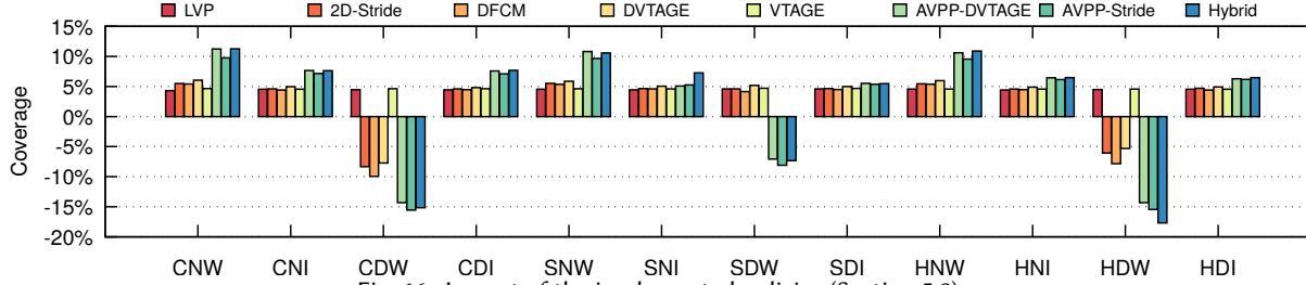
Fig. 16. Impact of the implemented policies (Section 5.3).
