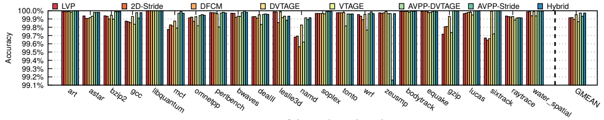
Fig. 10. Accuracy of the evaluated predictors.
