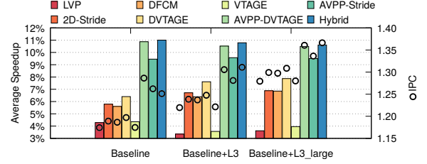
Fig. 22. Speedup of load value prediction with the three cache configurations shown in Table 5.
