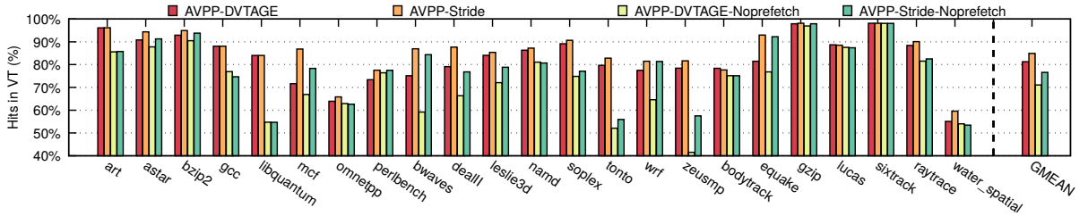
Fig. 15. VT hit rate with and without prefetching.
