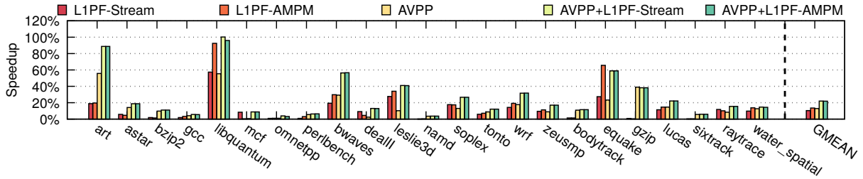
Fig. 24. Performance effect of L1 prefetching vs. AVPP.
