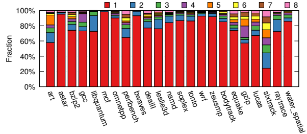
Fig. 20. AVPP prefetch distance distribution. The common case is distance=1 (i.e., to prefetch the next address), but other distances are also significant in some benchmarks.
