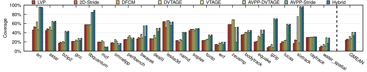
Fig. 9. Coverage of the evaluated predictors.
